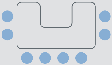
U-Shaped
